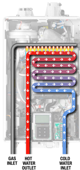
NPE-S2 Standard condensing tankless water heaters
